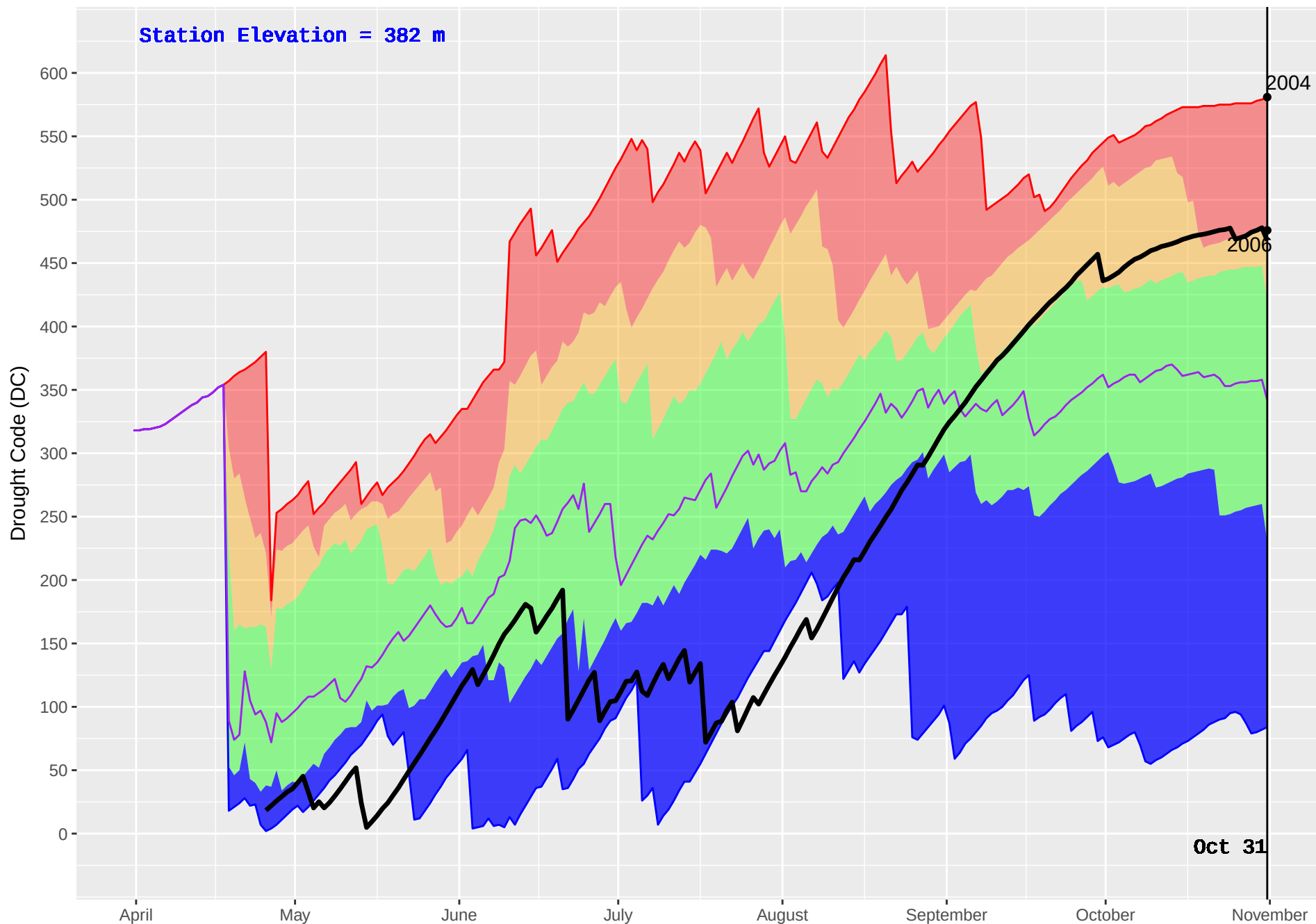
FORT NELSON FS (599) : Historical (1999–2016) and Current (2017) Noon Drought Code (DC)
