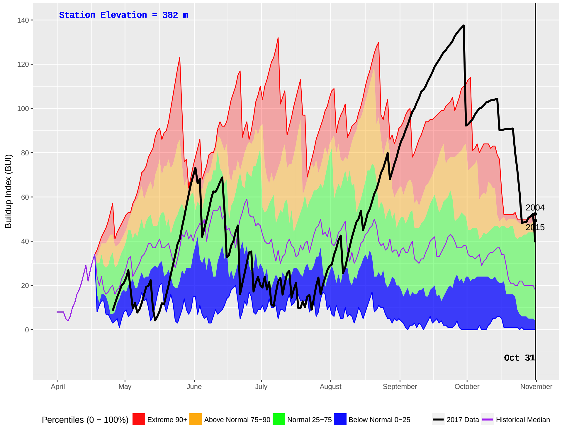
FORT NELSON FS (599) : Historical (1999–2016) and Current (2017) Noon Buildup Index (BUI)
