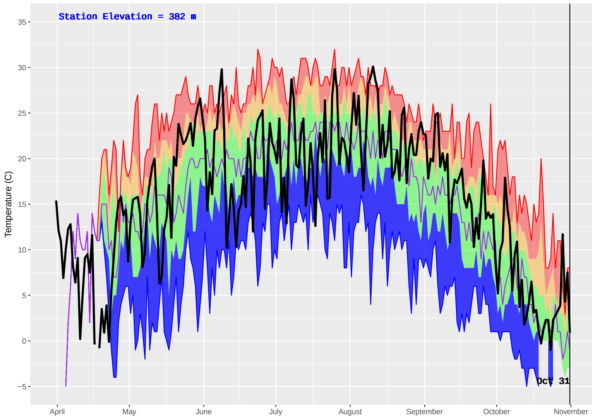
FORT NELSON FS (599) : Historical (1999–2016) and Current (2017) Noon Temperature
