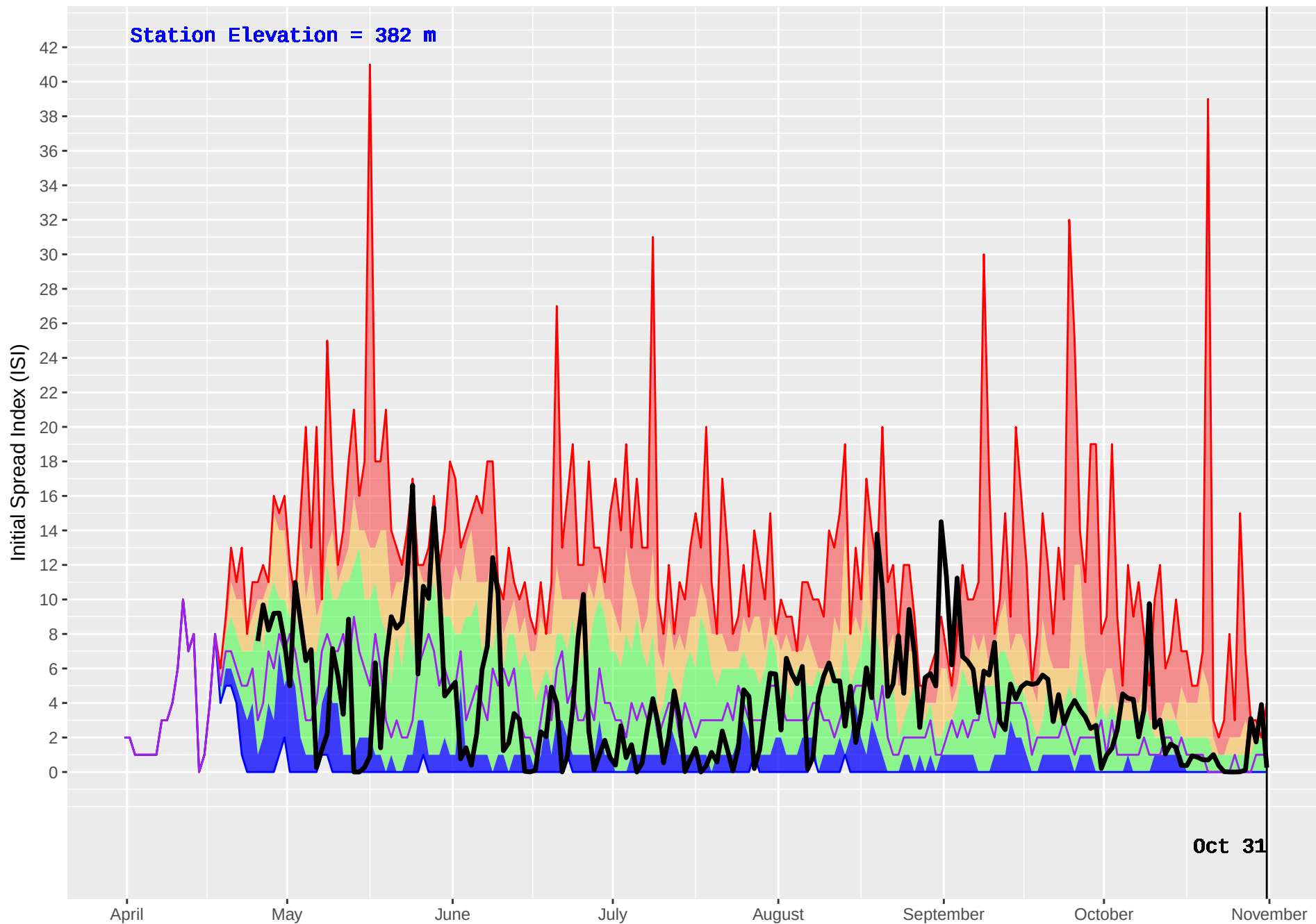
FORT NELSON FS (599) : Historical (1999–2016) and Current (2017) Noon Initial Spread Index (ISI)
